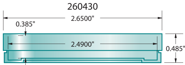
Note: All dimensions +/-0.020" unless otherwise noted
