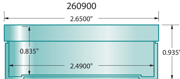
Note: All dimensions +/-0.020" unless otherwise noted
